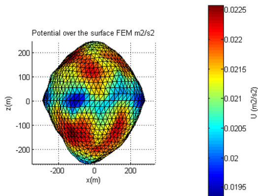
Figure 3. Potential over Bennu surface – FEM (xz view).
