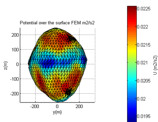
Figure 4. Potential over Bennu surface – FEM (yz view).
