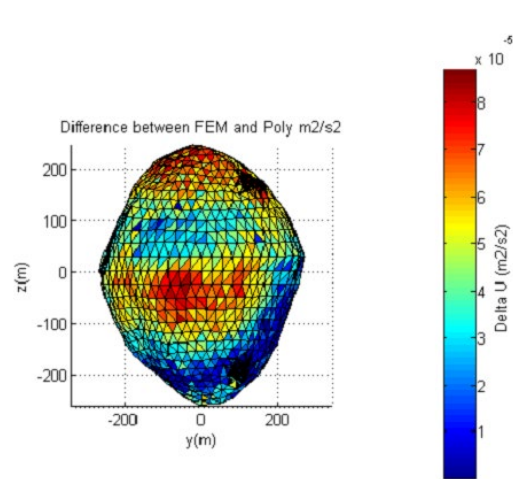
Figure 8. Potential difference over Benu surface (y-z view).
