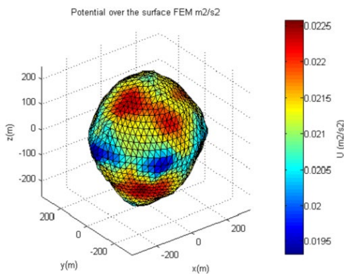
Figure 1. Potential over Bennu surface – FEM.
