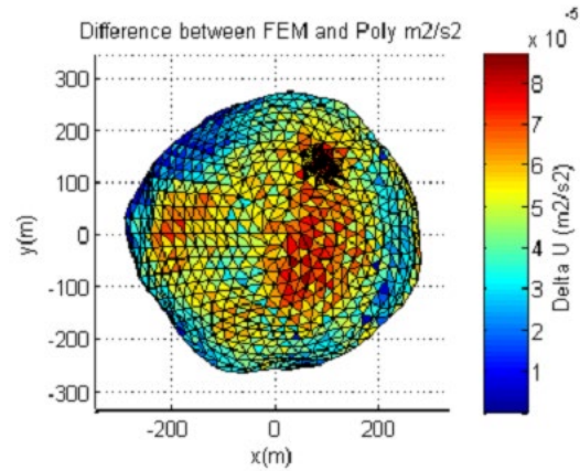
Figure 6. Potential difference over Benu surface (x-y view).
