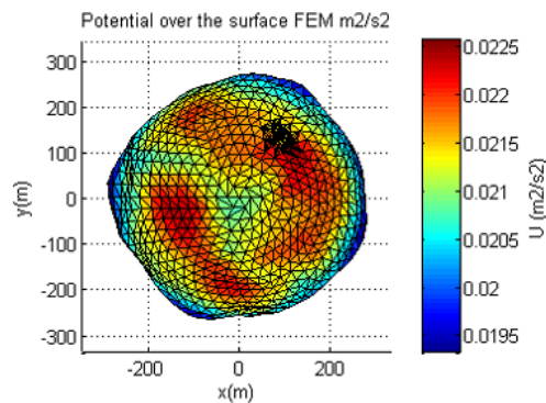
Figure 2. Potential over Bennu surface – FEM (xy view).
