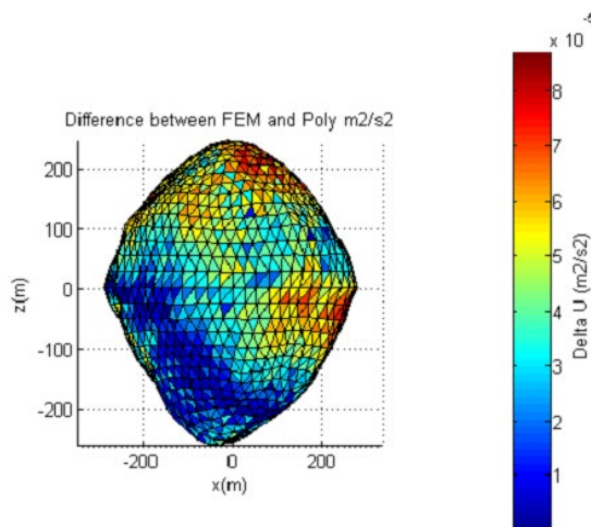
Figure 7. Potential difference over Benu surface (x-z view).
