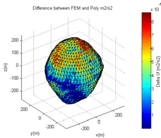
Figure 5. Potential difference over Benu surface.
